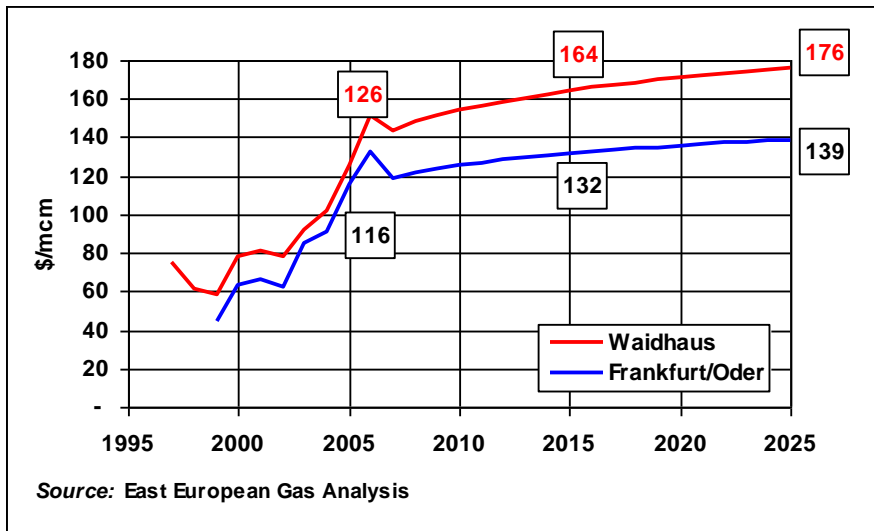
Figure 3.17: Cost of Gas Delivered to German Border
